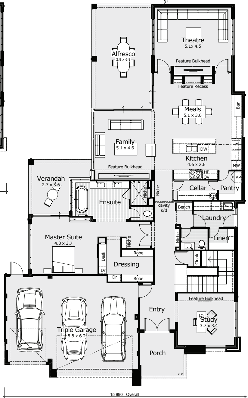
GROUND FLOOR
